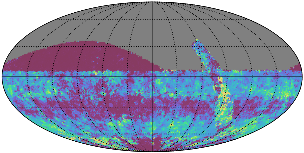
retro_baseline_v2.0_10yrs All sky gr bands: 75th Percentile Intranight Timespan
