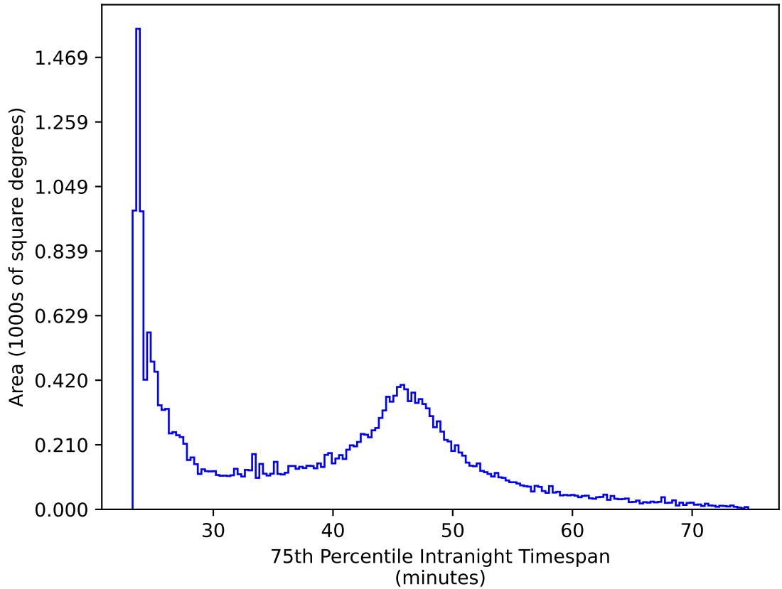
retro_baseline_v2.0_10yrs All sky gr bands: 75th Percentile Intranight Timespan
