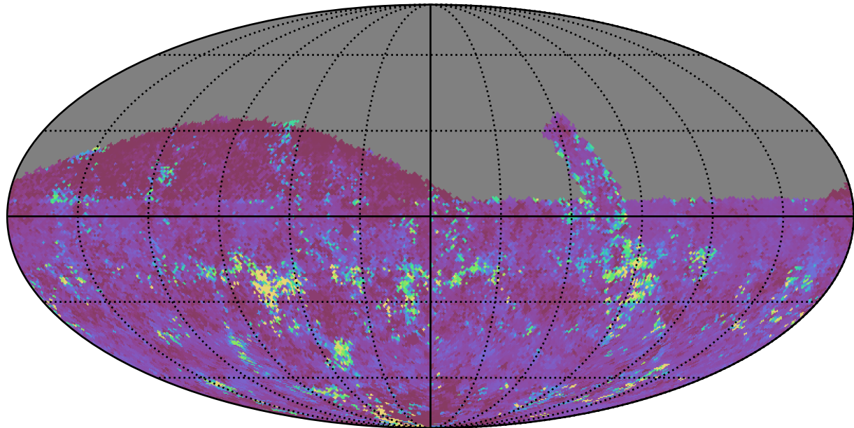
retro_baseline_v2.0_10yrs All sky g band: 75th Percentile Intranight Timespan
