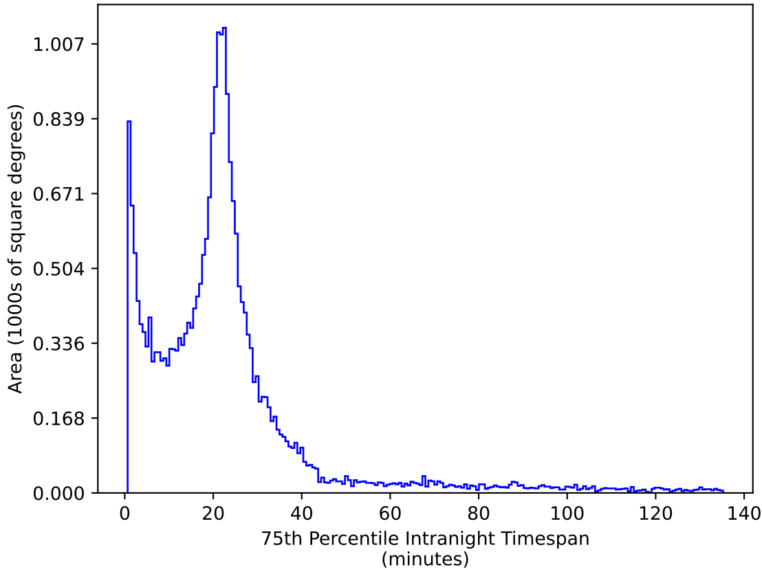
retro_baseline_v2.0_10yrs All sky g band: 75th Percentile Intranight Timespan
