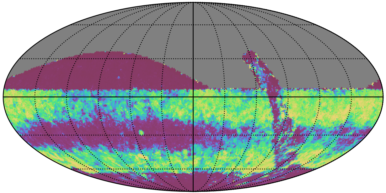
retro_baseline_v2.0_10yrs All sky all bands: 75th Percentile Intranight Timespan
