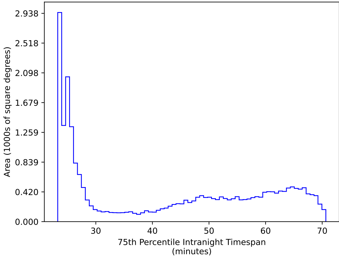
retro_baseline_v2.0_10yrs All sky all bands: 75th Percentile Intranight Timespan
