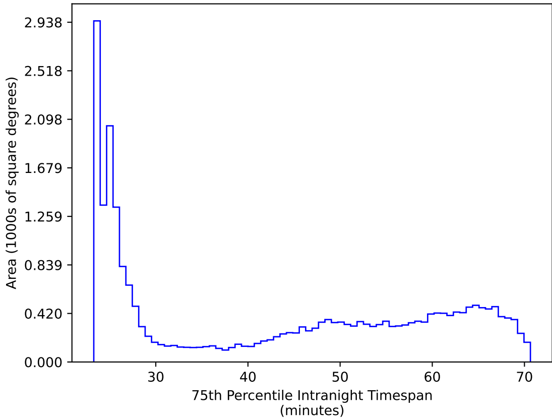
retro_baseline_v2.0_10yrs All sky: 75th Percentile Intranight Timespan
