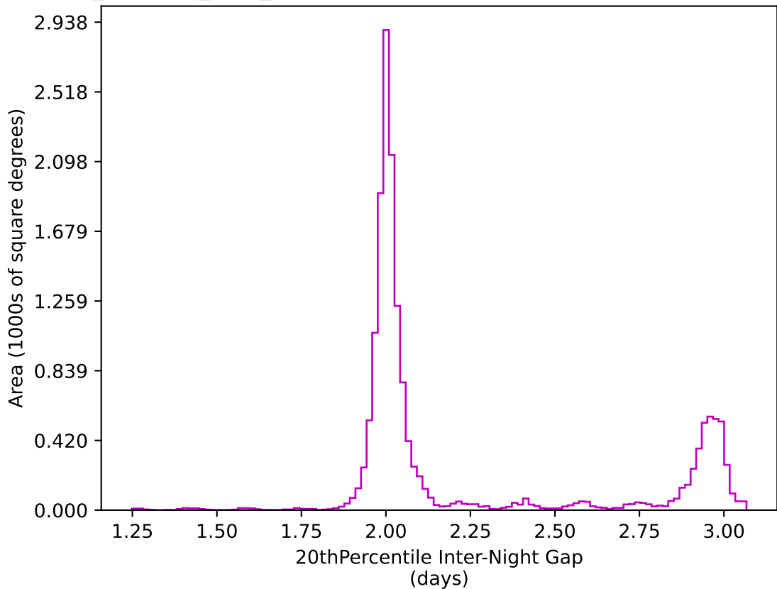
retro_baseline_v2.0_10yrs WFD z band: 20thPercentile Inter-Night Gap
