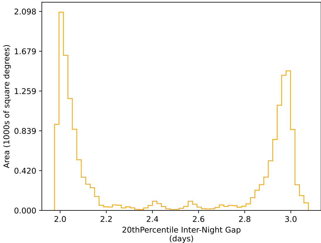
retro_baseline_v2.0_10yrs WFD r band: 20thPercentile Inter-Night Gap
