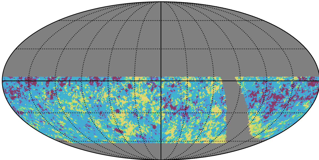
retro_baseline_v2.0_10yrs WFD i band: 20thPercentile Inter-Night Gap
