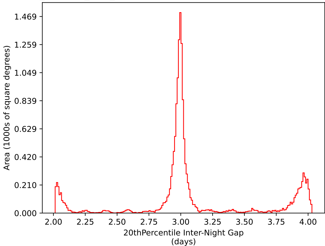
retro_baseline_v2.0_10yrs WFD i band: 20thPercentile Inter-Night Gap
