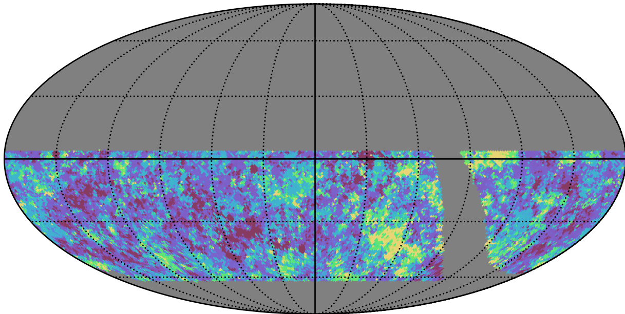
retro_baseline_v2.0_10yrs WFD g band: 20thPercentile Inter-Night Gap
