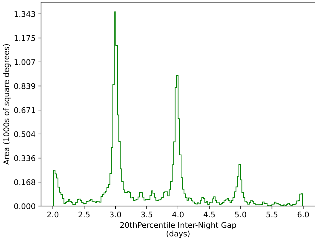
retro_baseline_v2.0_10yrs WFD g band: 20thPercentile Inter-Night Gap
