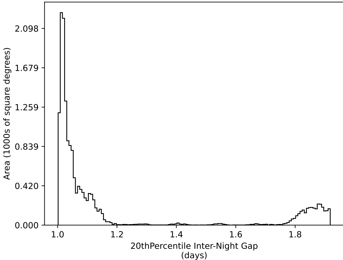
retro_baseline_v2.0_10yrs WFD all bands: 20thPercentile Inter-Night Gap
