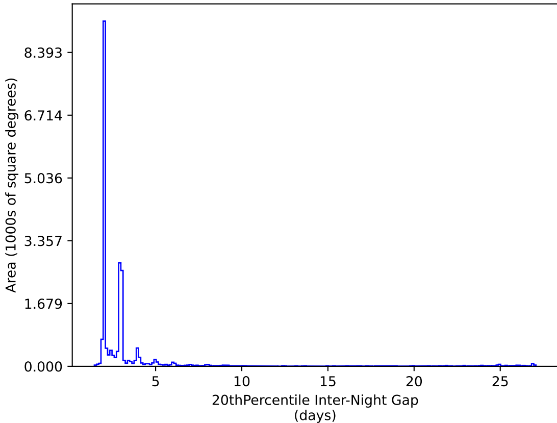
retro_baseline_v2.0_10yrs All sky y band: 20thPercentile Inter-Night Gap
