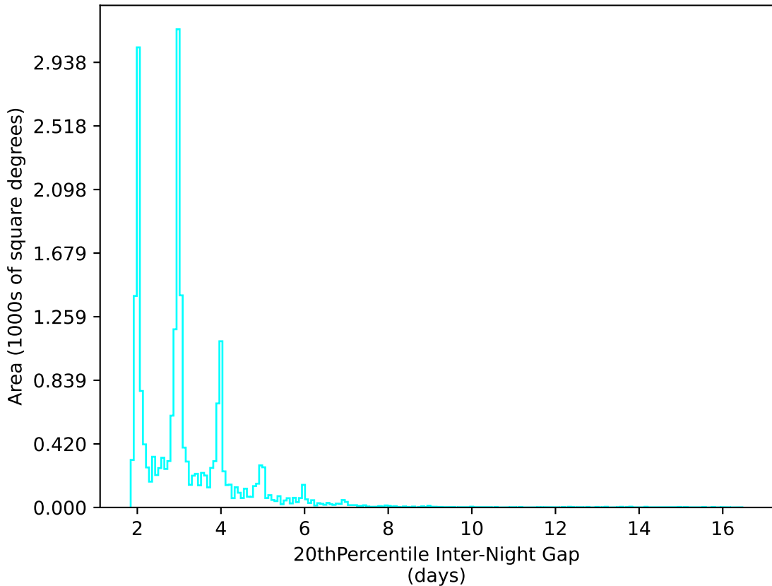
retro_baseline_v2.0_10yrs All sky u band: 20thPercentile Inter-Night Gap
