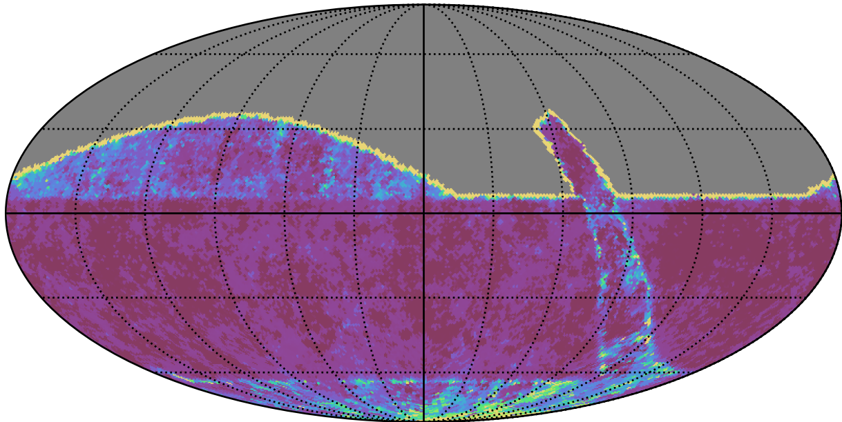
retro_baseline_v2.0_10yrs All sky r band: 20thPercentile Inter-Night Gap
