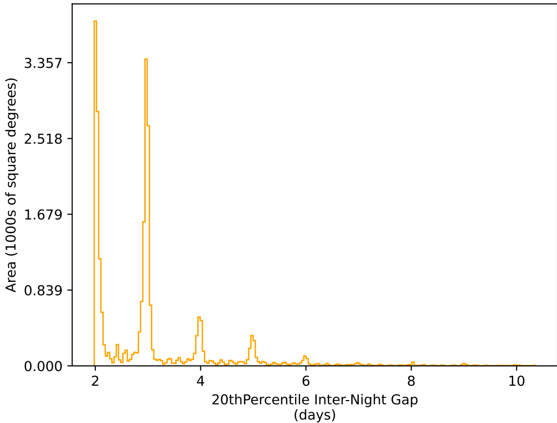
retro_baseline_v2.0_10yrs All sky r band: 20thPercentile Inter-Night Gap
