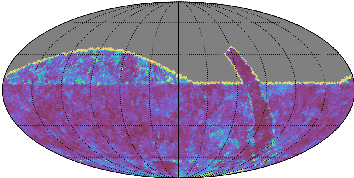
retro_baseline_v2.0_10yrs All sky g band: 20thPercentile Inter-Night Gap
