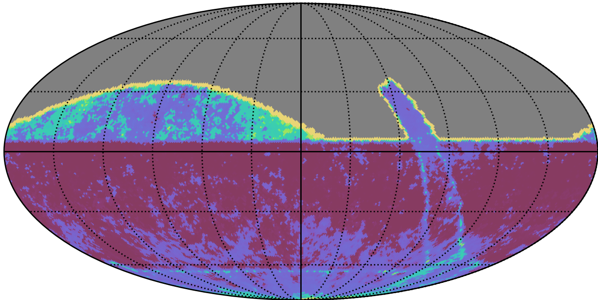
retro_baseline_v2.0_10yrs All sky all bands: 20thPercentile Inter-Night Gap
