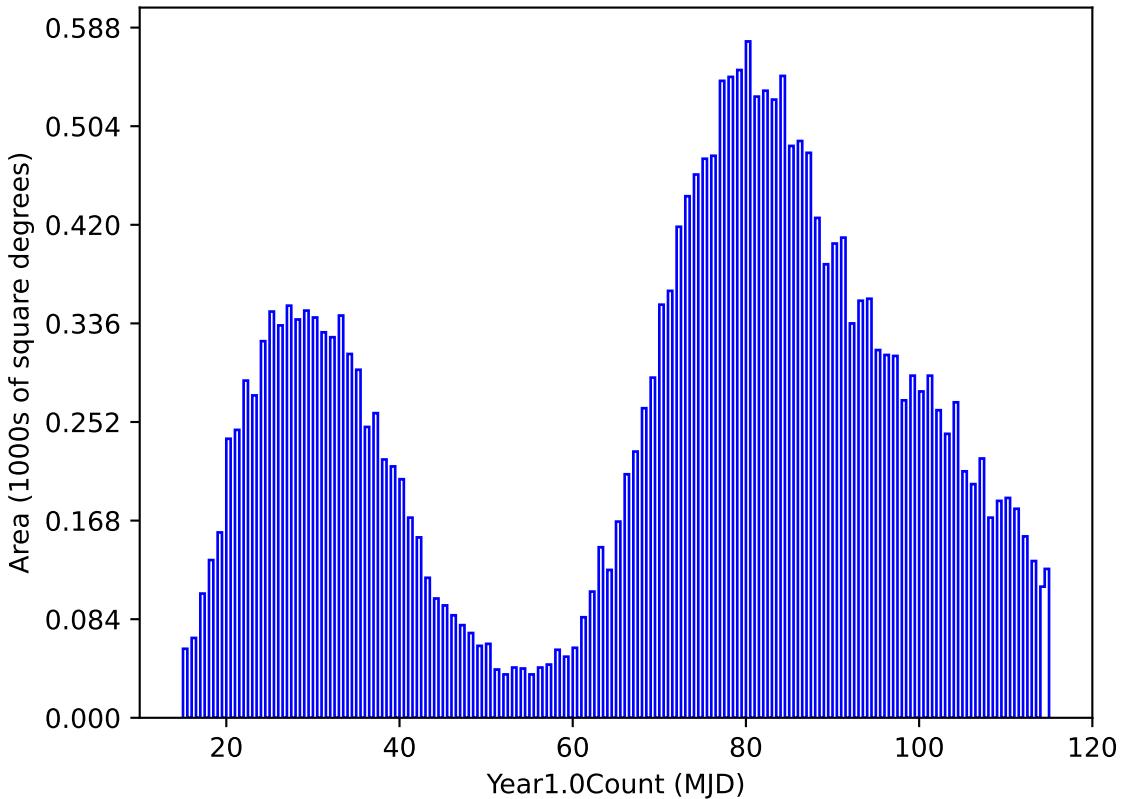
retro_baseline_v2.0_10yrs night < 365.25: Year1.0Count
