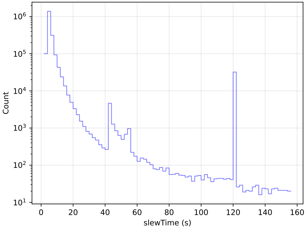
retro_baseline_v2.0_10yrs All visits: Slew Time Histogram
