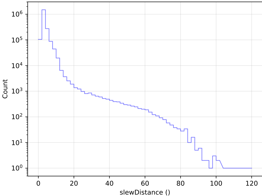
retro_baseline_v2.0_10yrs All visits: Slew Distance Histogram
