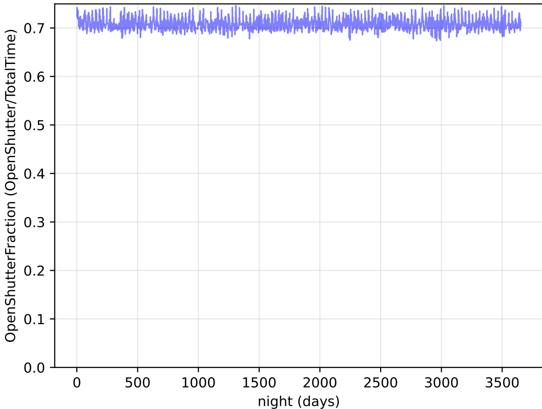
retro_baseline_v2.0_10yrs : OpenShutterFraction
