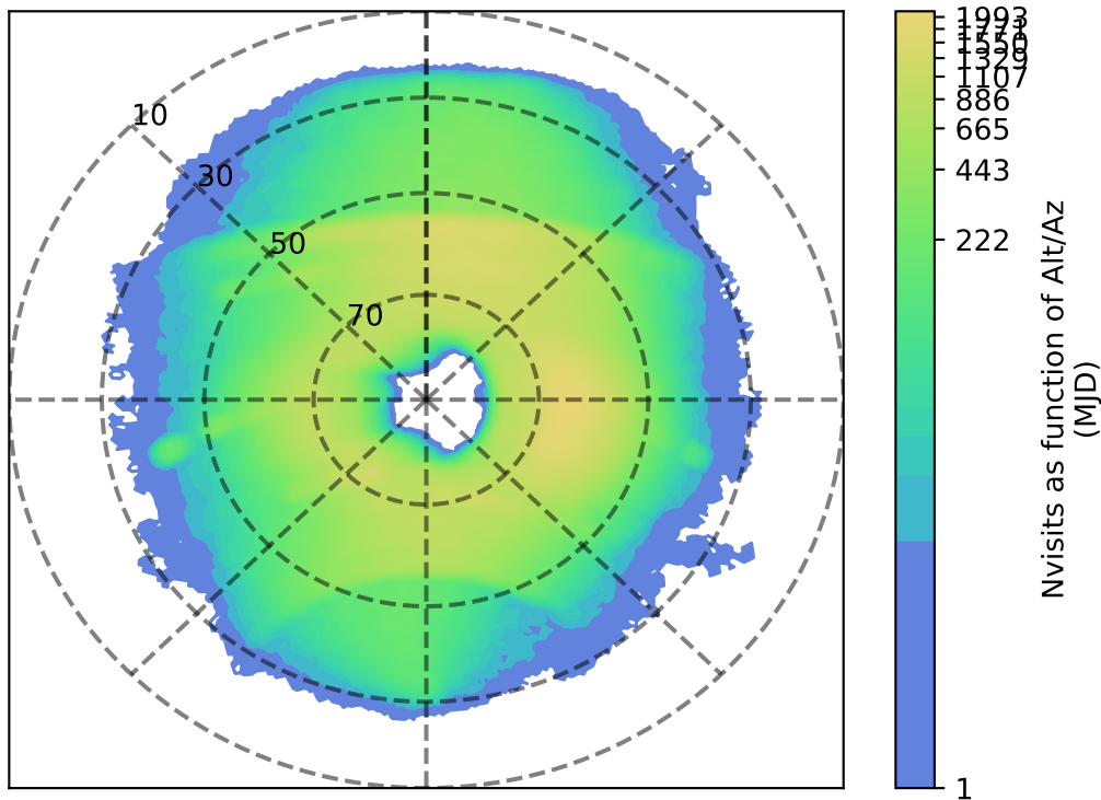
retro_baseline_v2.0_10yrs z: Nvisits as function of Alt/Az
