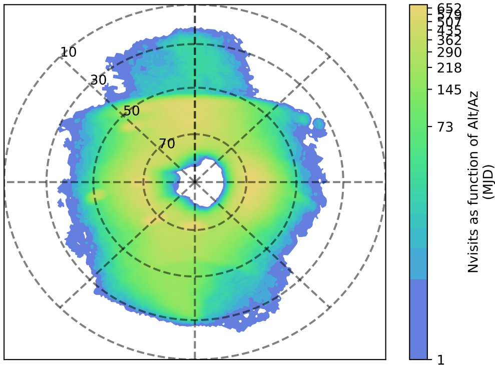
retro_baseline_v2.0_10yrs u: Nvisits as function of Alt/Az
