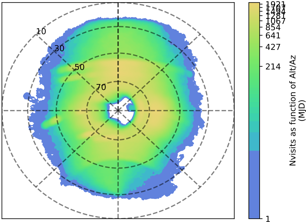
retro_baseline_v2.0_10yrs r: Nvisits as function of Alt/Az
