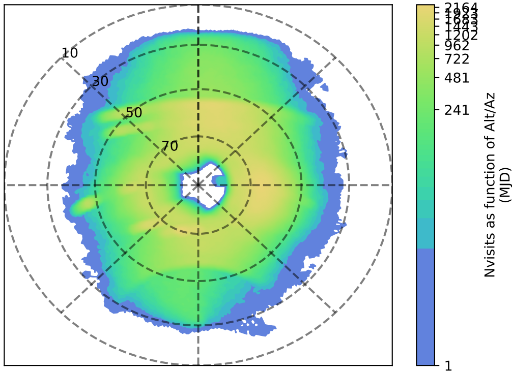
retro_baseline_v2.0_10yrs i: Nvisits as function of Alt/Az
