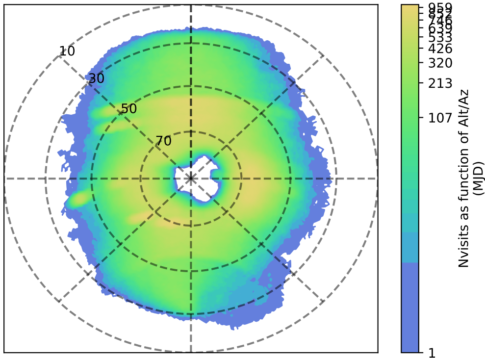
retro_baseline_v2.0_10yrs g: Nvisits as function of Alt/Az
