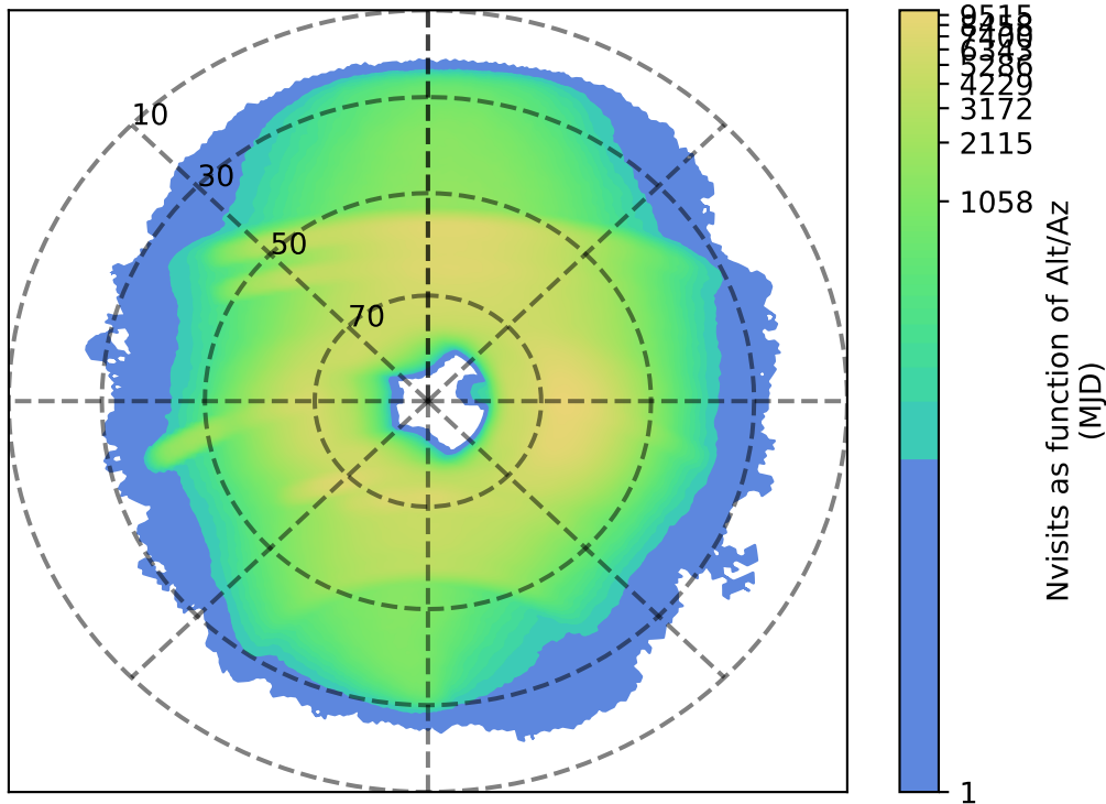
retro_baseline_v2.0_10yrs : Nvisits as function of Alt/Az
