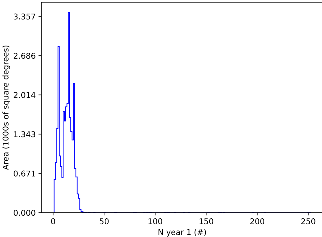
retro_baseline_v2.0_10yrs z and night < 365: N year 1
