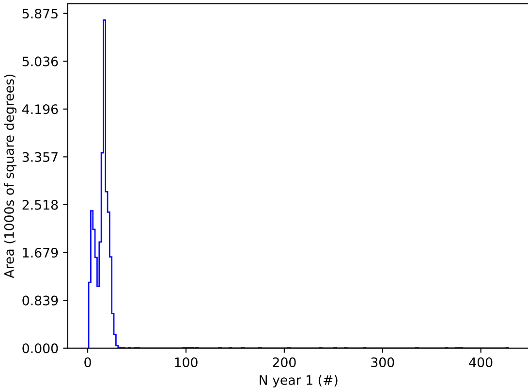
retro_baseline_v2.0_10yrs i and night < 365: N year 1
