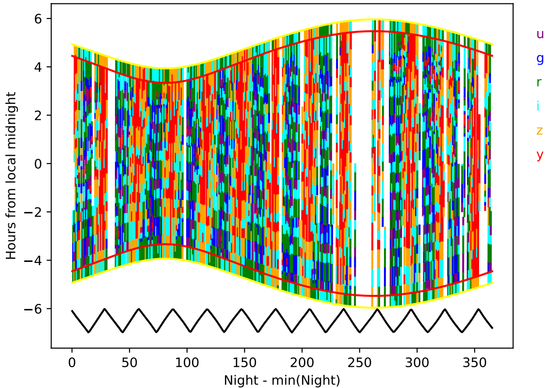
retro_baseline_v2.0_10yrs year 9-10: Hourglass
