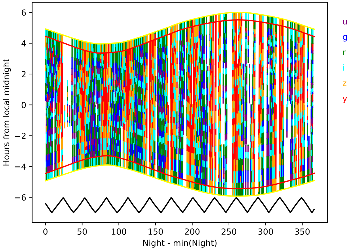
retro_baseline_v2.0_10yrs year 4-5: Hourglass
