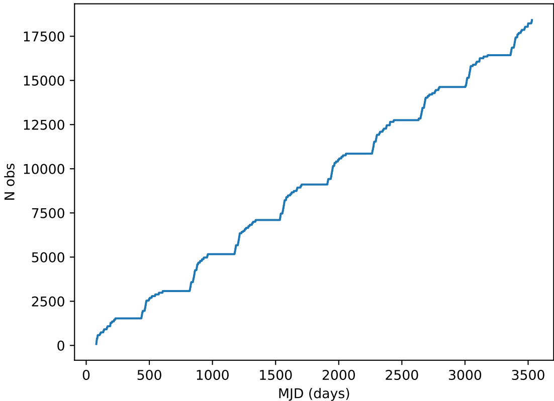
retro_baseline_v2.0_10yrs note like DD:COSMOS%: Cumulative
