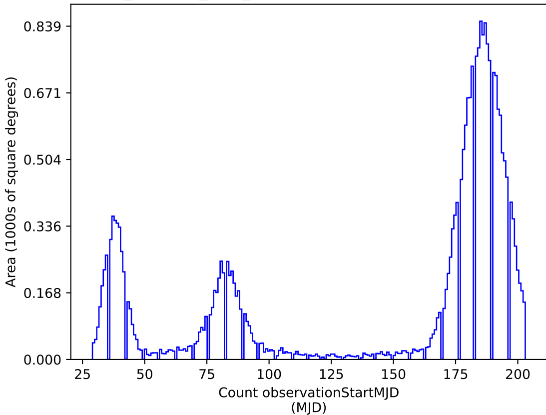
retro_baseline_v2.0_10yrs i: Count observationStartMJD
