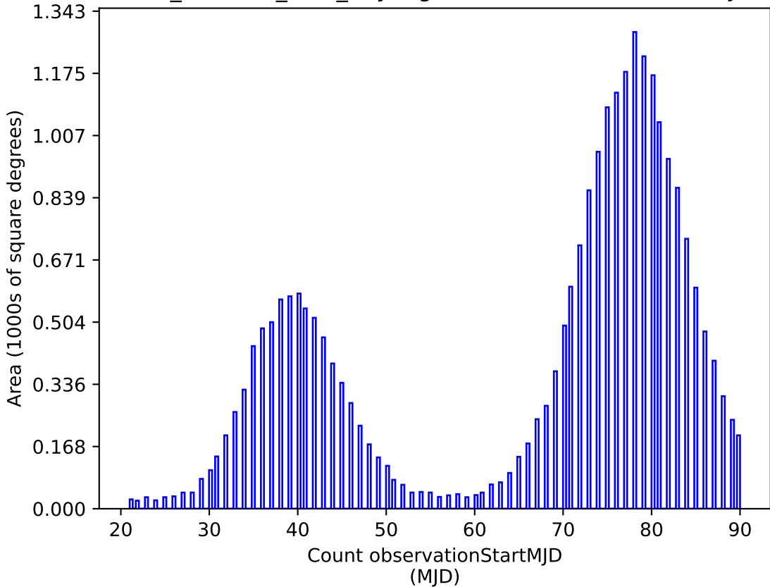
retro_baseline_v2.0_10yrs g: Count observationStartMJD
