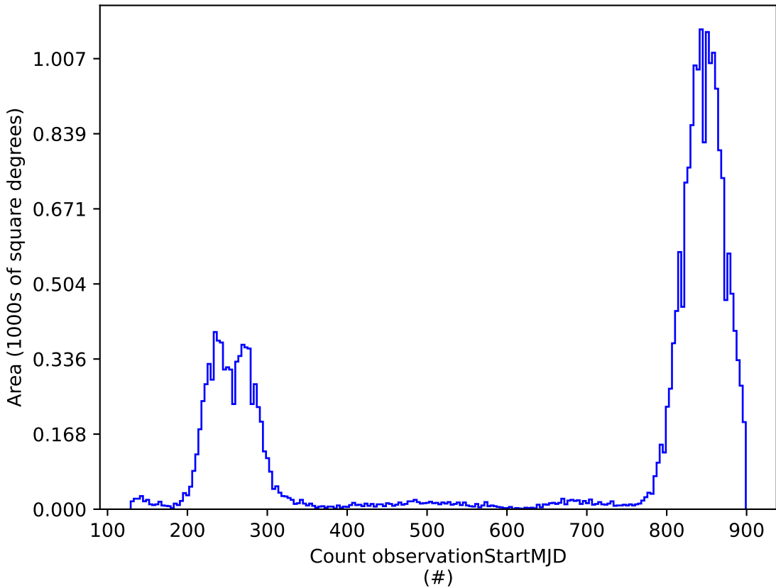
retro_baseline_v2.0_10yrs : Count observationStartMJD
