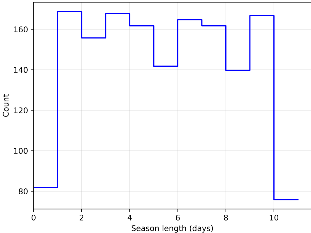
retro_baseline_v2.0_10yrs DD:XMM_LSS all bands: SeasonLength
