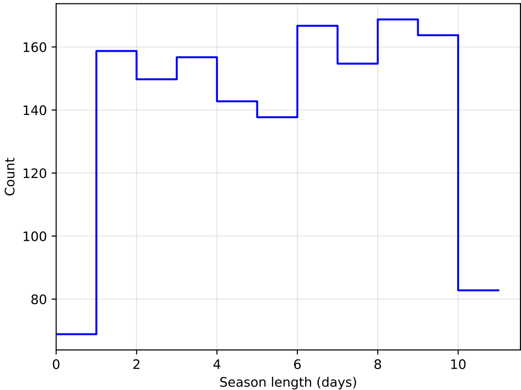
retro_baseline_v2.0_10yrs DD:ELAISS1 all bands: SeasonLength
