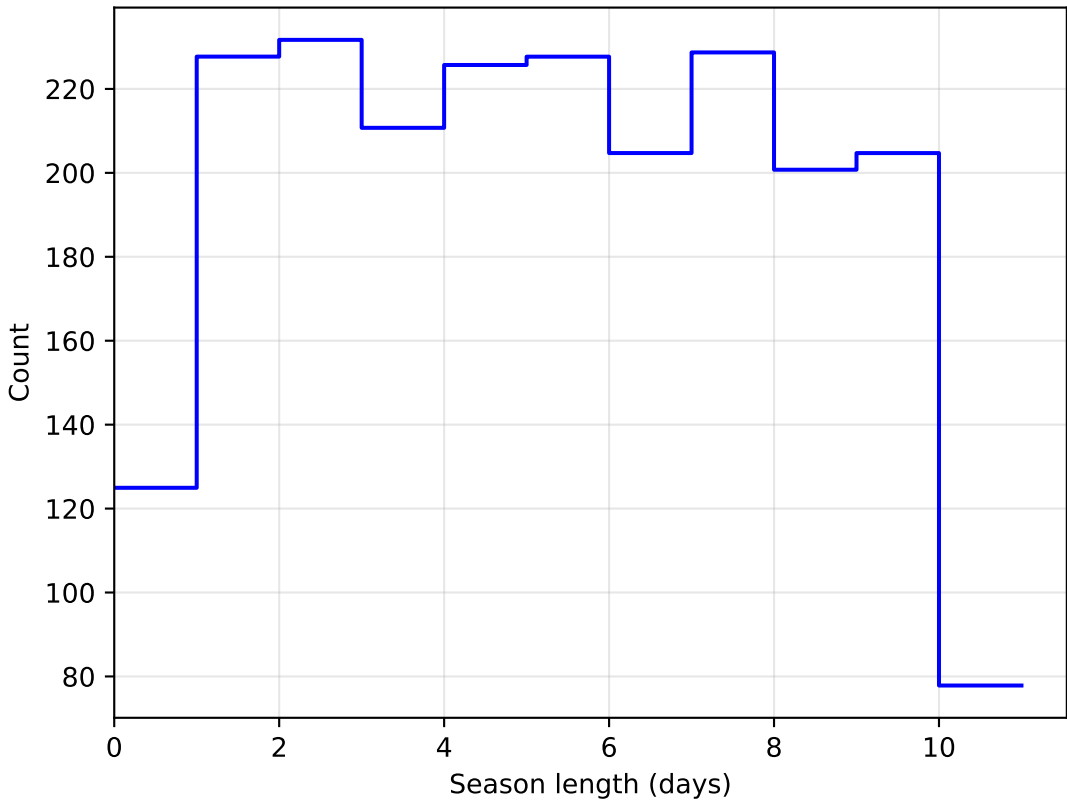
retro_baseline_v2.0_10yrs DD:ECDFS all bands: SeasonLength
