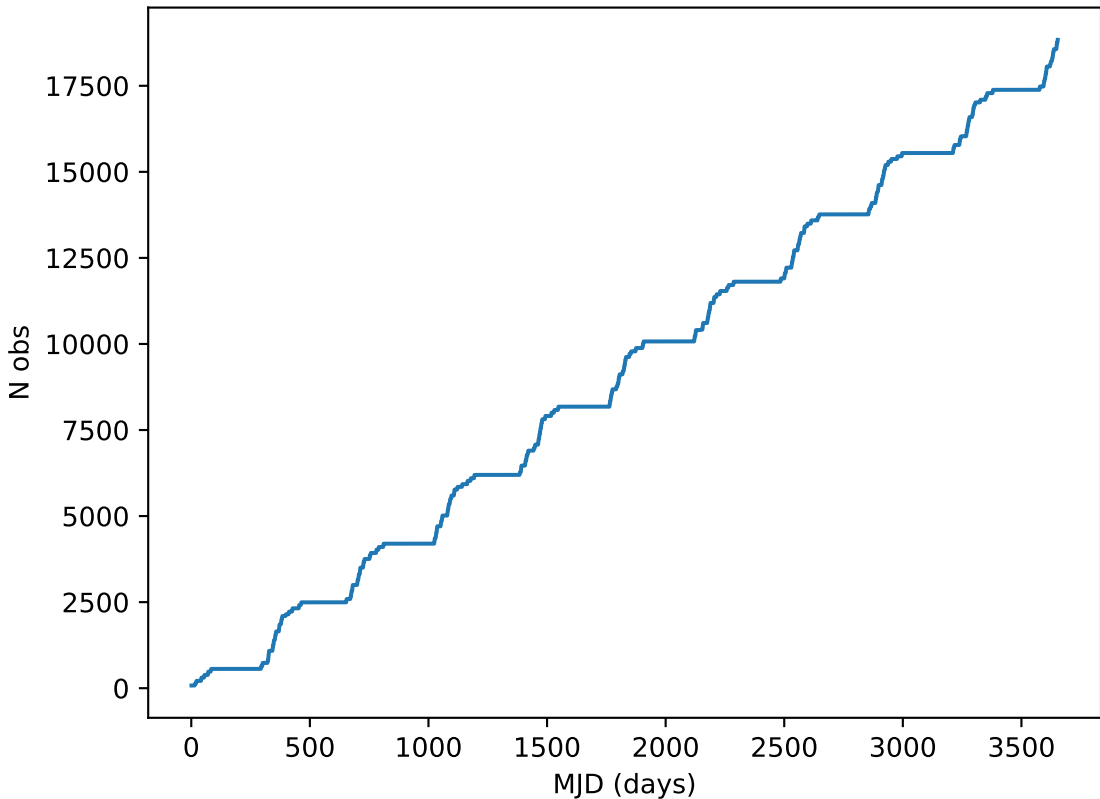
retro_baseline_v2.0_10yrs all bands: DD:XMM_LSS Cumulative NVisits
