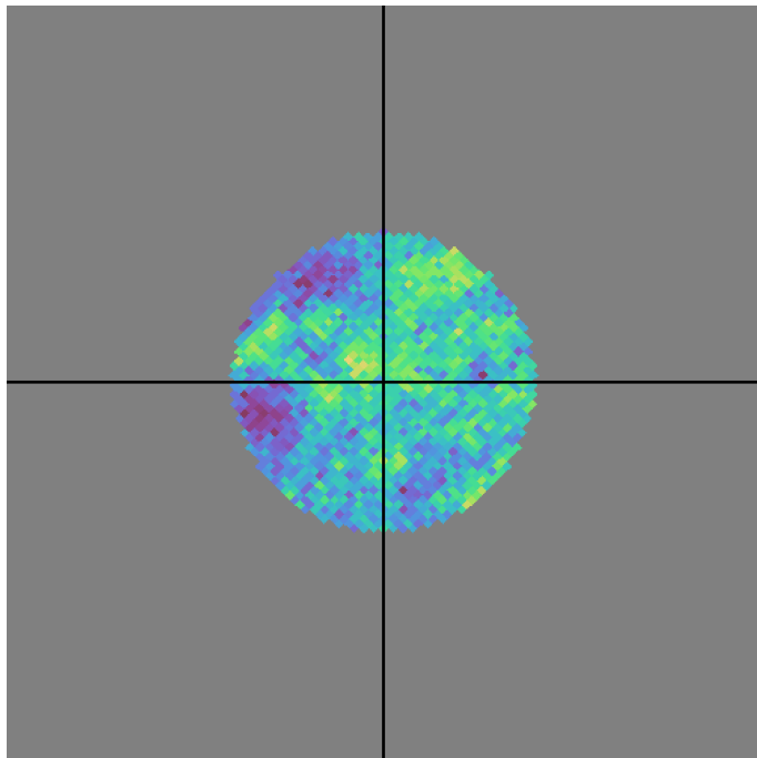
retro_baseline_v2.0_10yrs g band: DD:WFD NVisits
