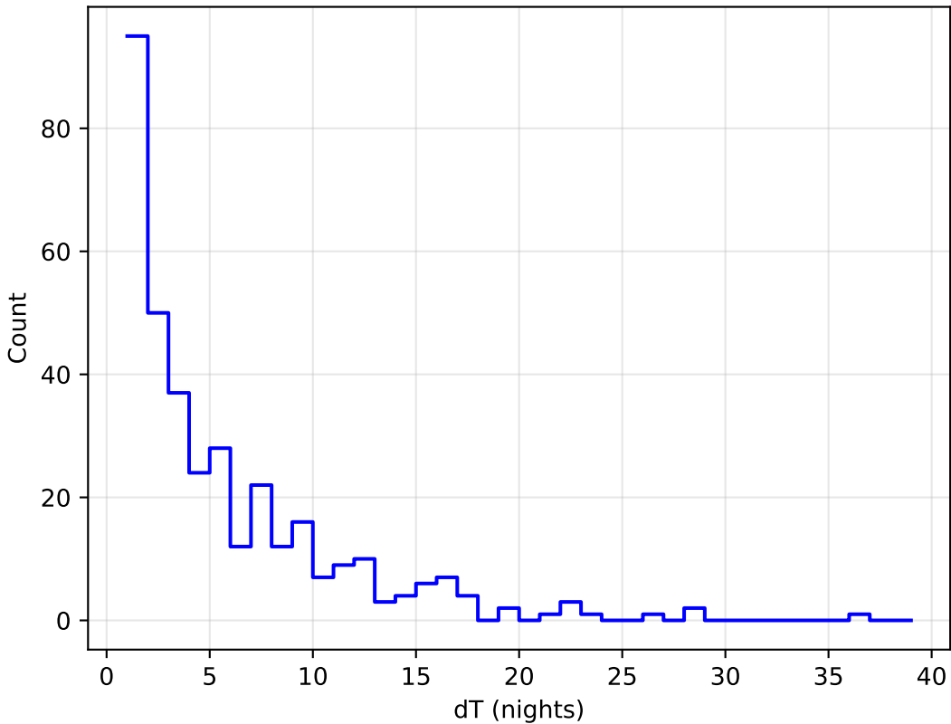
retro_baseline_v2.0_10yrs all bands: DD:WFD Delta Nights Histogram
