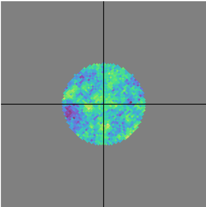
retro_baseline_v2.0_10yrs g band: DD:WFD CoaddM5
