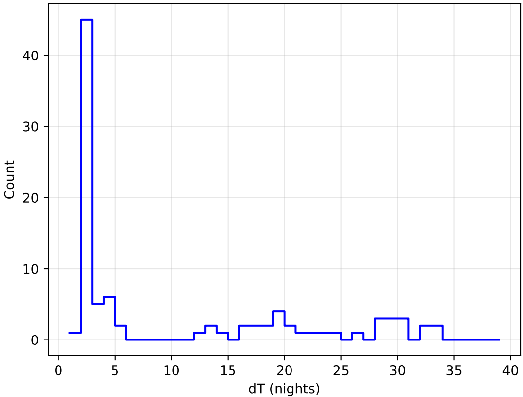
retro_baseline_v2.0_10yrs all bands: DD:EDFS Delta Nights Histogram
