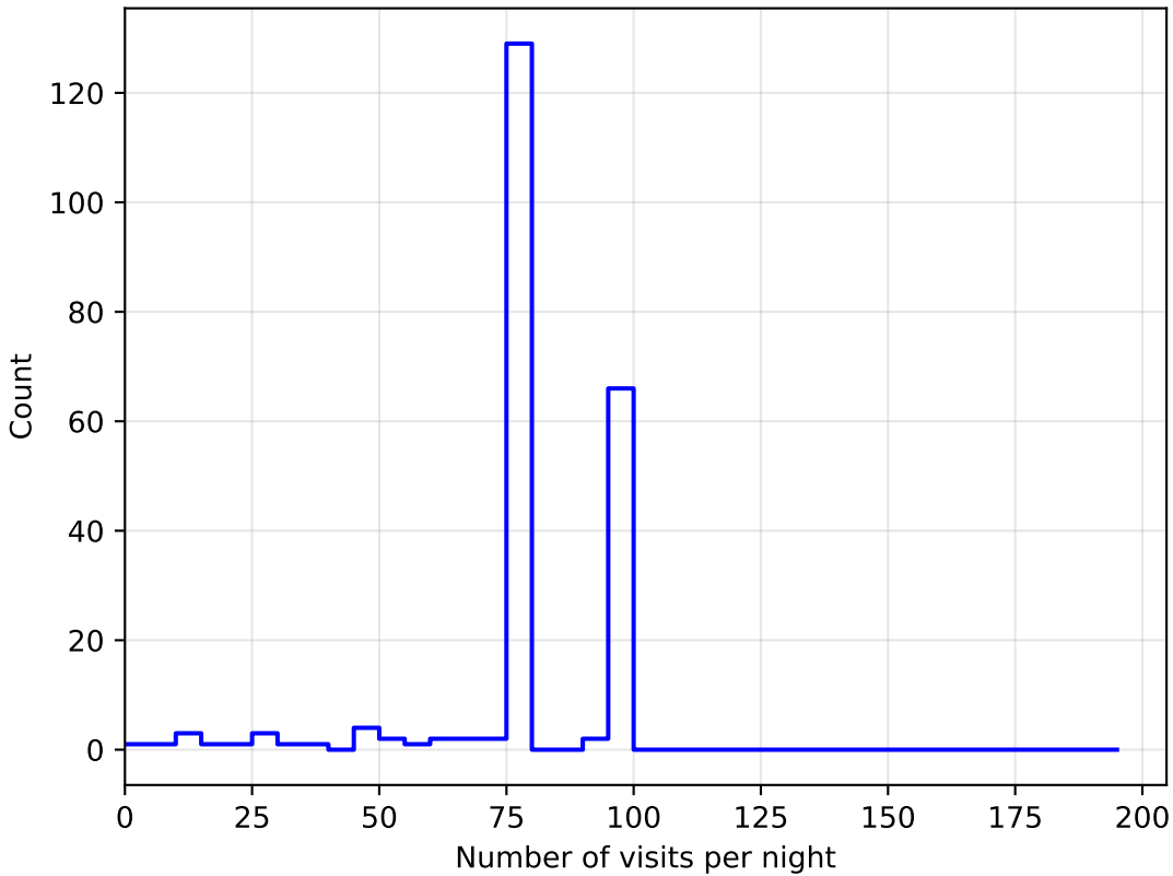
retro_baseline_v2.0_10yrs all bands: DD:ECDFS NVisitsPerNight
