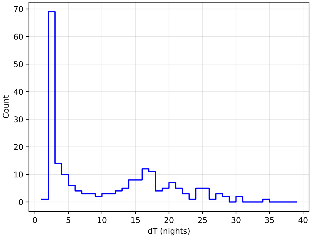
retro_baseline_v2.0_10yrs all bands: DD:ECDFS Delta Nights Histogram
