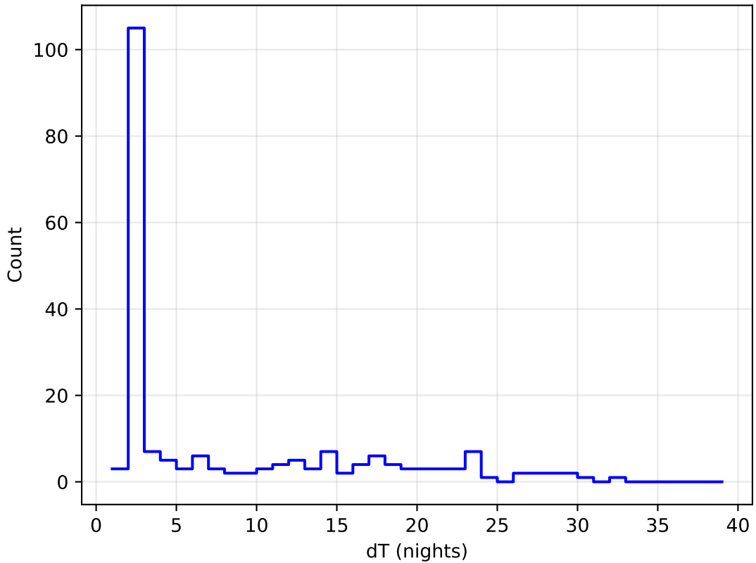
retro_baseline_v2.0_10yrs all bands: DD: COSMOS Delta Nights Histogram
