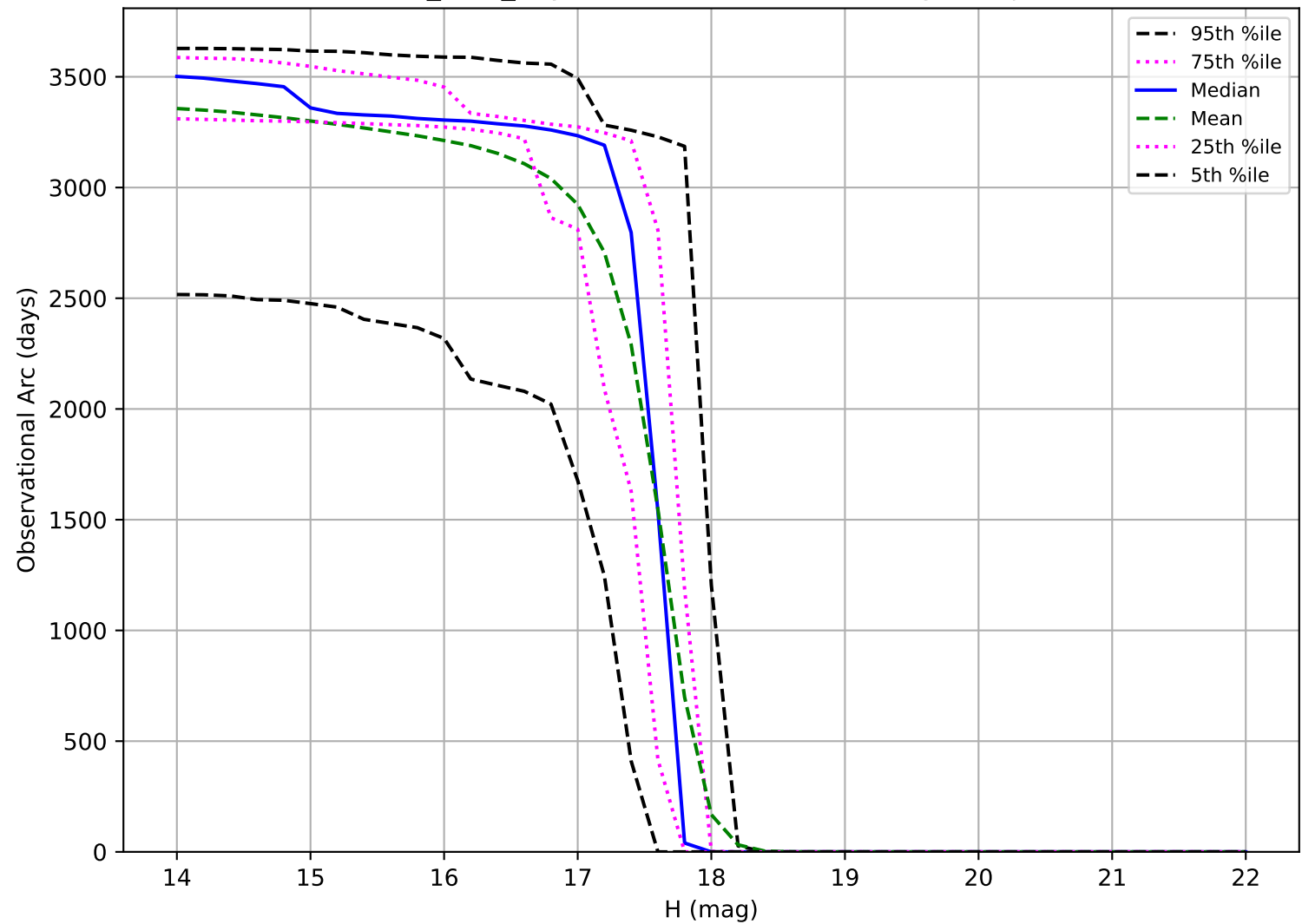
octo_v3.4_10yrs: Observational Arc Length Trojan
